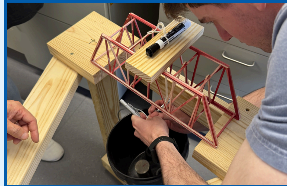
Balsa Wood Bridge First Place
